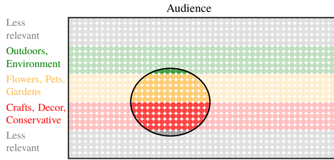
Figure 1: Single-ad blob
